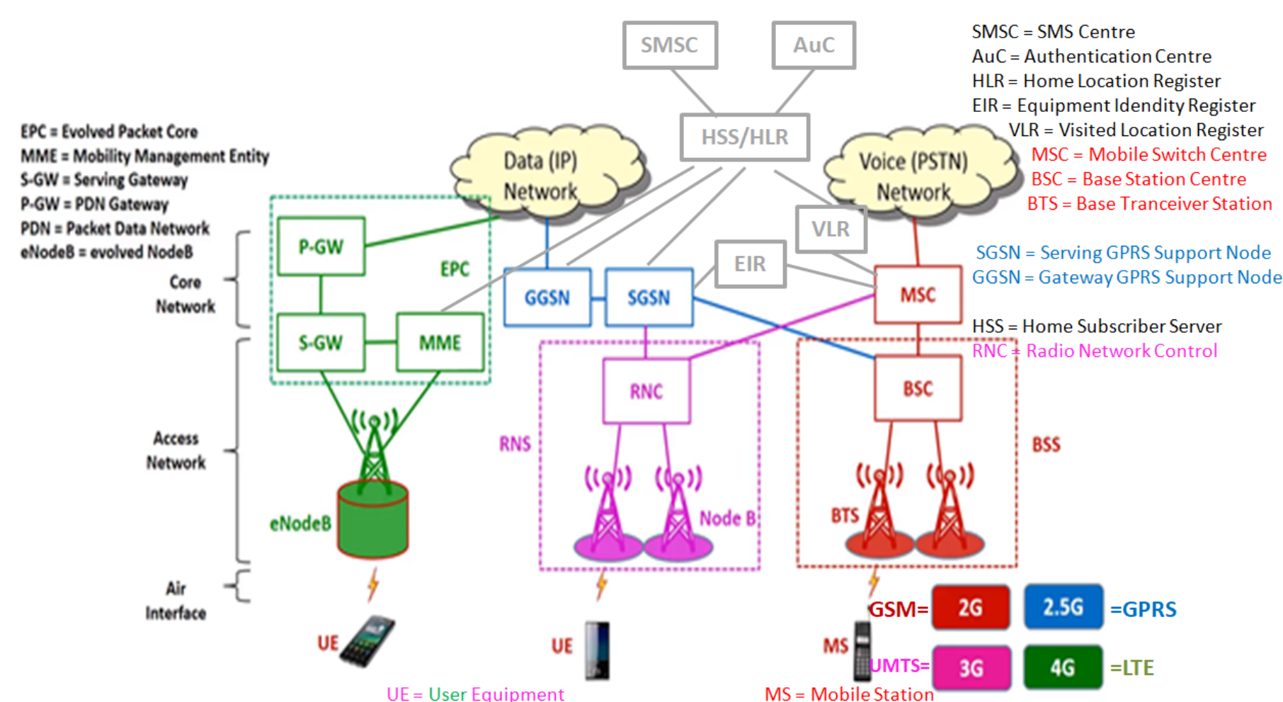
Figure 1: 2G, 3G and 4G Networks
