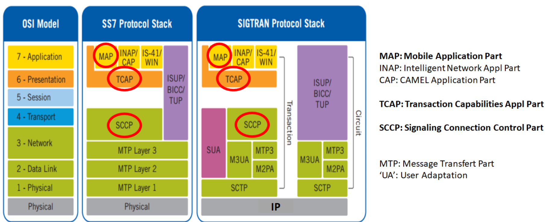
Figure 2: SS7 and SIGTRAN protocol stacks
