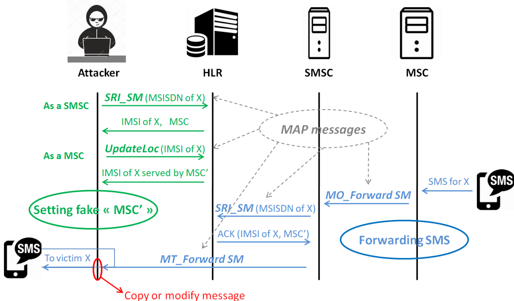
Figure 3: SMS interception
