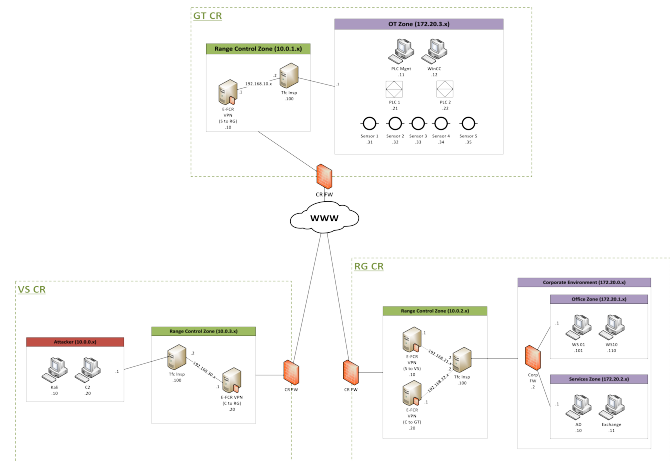
Figure 5. Network diagram of the training scenario
