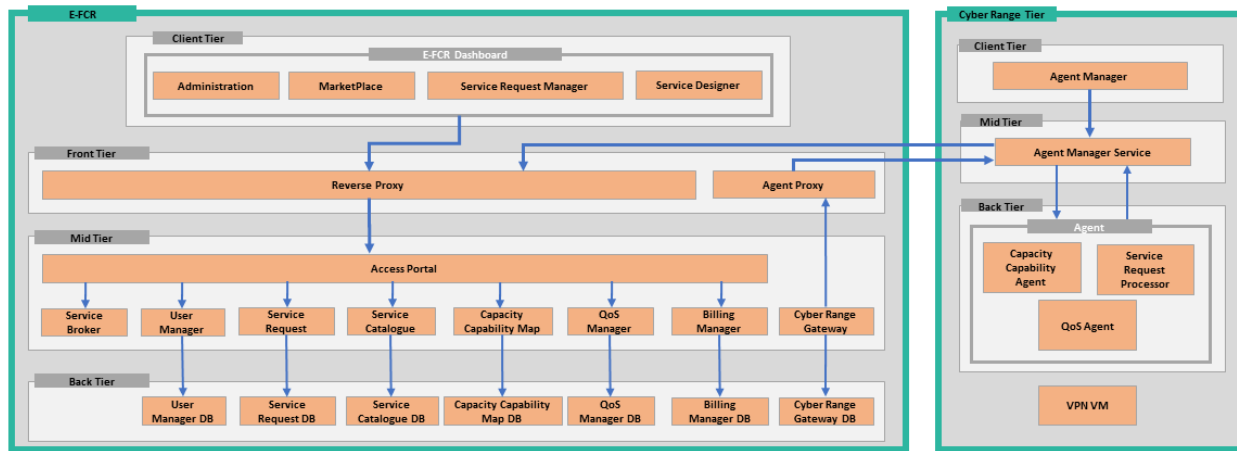
Figure 2. E-FCR architecture
